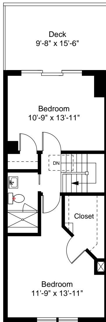
Second Floor Plan Ceiling Height = 7'-5"
