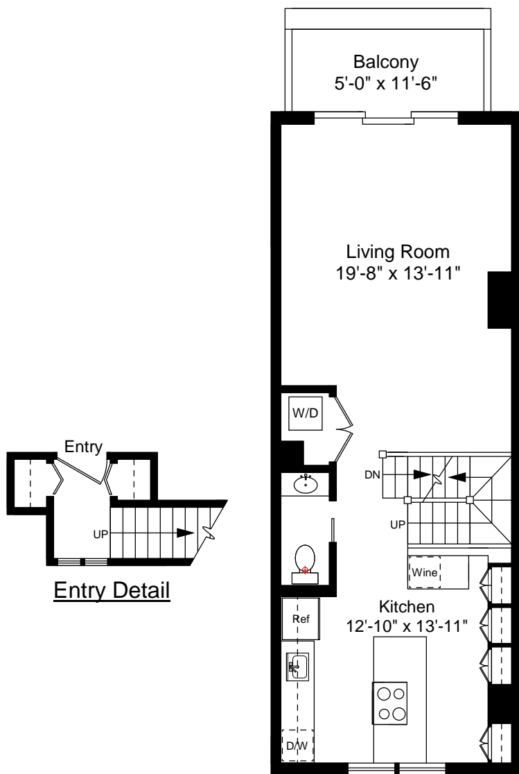
First Floor Plan Ceiling Height = 7'-8"
